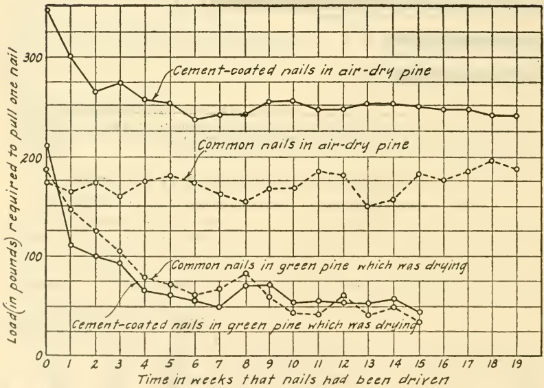
FIGURE 21.—Effect of changes in moisture content with time on holding power of sevenpenny nails driven to \frac{1}{2} -inch depth
